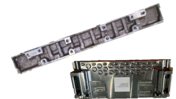
BATTERY BOX COMPONENTS FORGING/MACHINING
