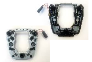
AIRBAG FRAME METAL FORMING / PLASTIC OVERMOULDING
