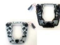
AIRBAG FRAME METAL FORMING / PLASTIC OVERMOULDING
